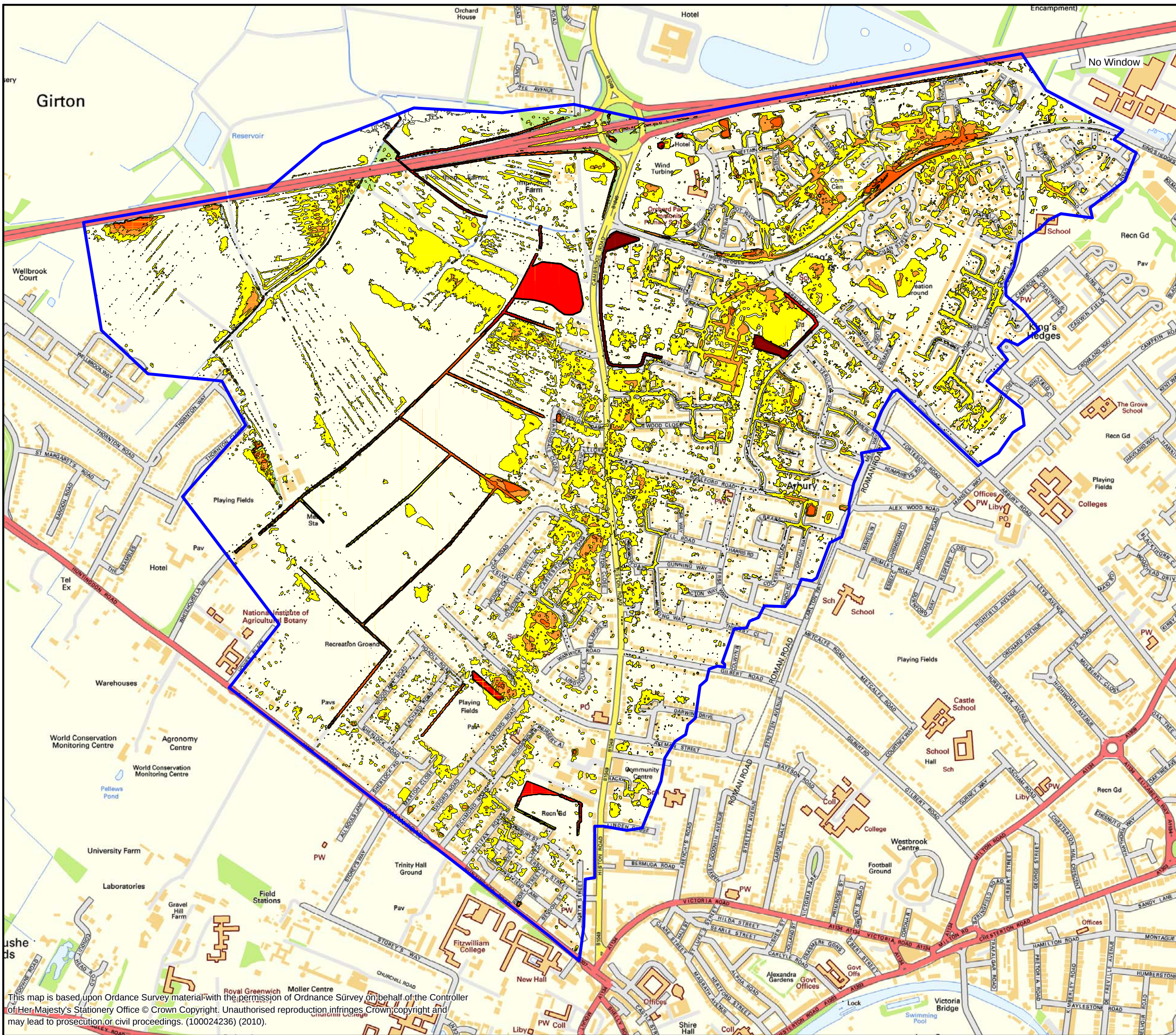
FIGURE F7 0.5% AEP "ENGINEERING OPTION C1" PLUVIAL MODELLING MAXIMUM DEPTH KING'S HEDGES AND ARBURY
